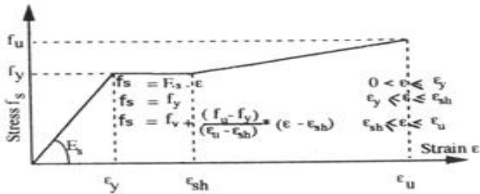
Trilinear Stress-Strain Curve for Steel Reinforcement in Tension and Compression
