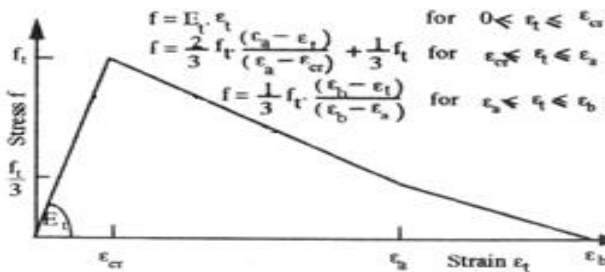
Trilinear Model for Concrete in Tension
