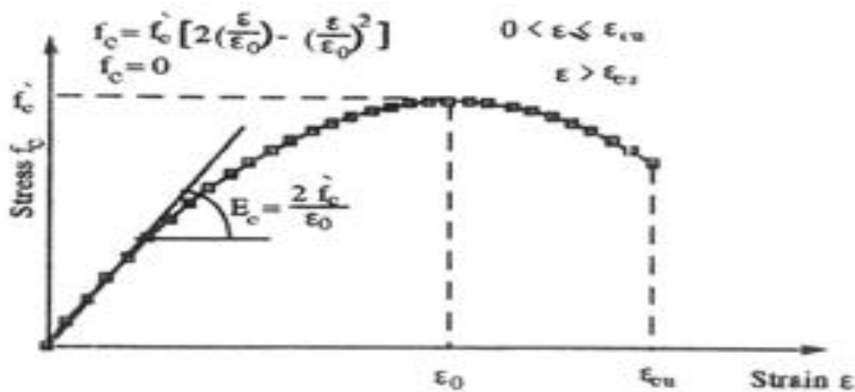
Concrete Stress-Strain Curve in Compression
